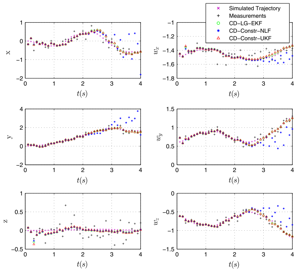
Fig. 5 Example of generated trajectory, measurements, CD-Constr-NLF output and CD-LG-EKF output with [x, y, z]^T = T and [w_x, w_y, w_z]^T = [\log_{SO(3)}(R)]_{SO(3)}^\vee
